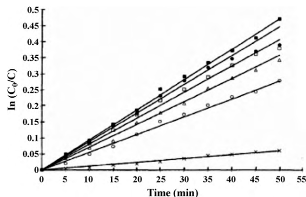
Fig. 5. \ln C_0/C vs. t for copper deposition during constant current electrolysis. Vibration velocity, cm/s: (X) – 0 (natural convection); (○) – 4.2; (△) – 6.3; (□) – 8.4; (●) – 12.6; (■) – 16.8.
