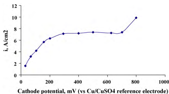
Fig. 3. Typical polarization curve for the deposition of copper under natural convection from 0.1 M \text{CuSO}_4 in 0.5 M \text{H}_2\text{SO}_4 .
