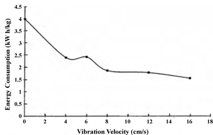
Fig. 13. Effect of vibration velocity on the energy consumption of copper deposition.
