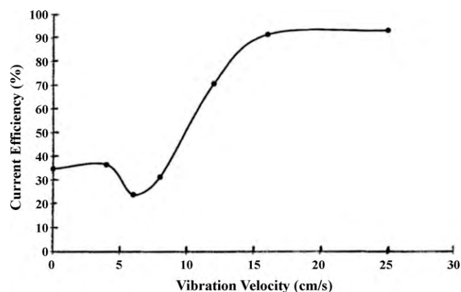
Fig. 12. Effect of vibration velocity on the current efficiency of FeSO 4 anodic oxidation.
