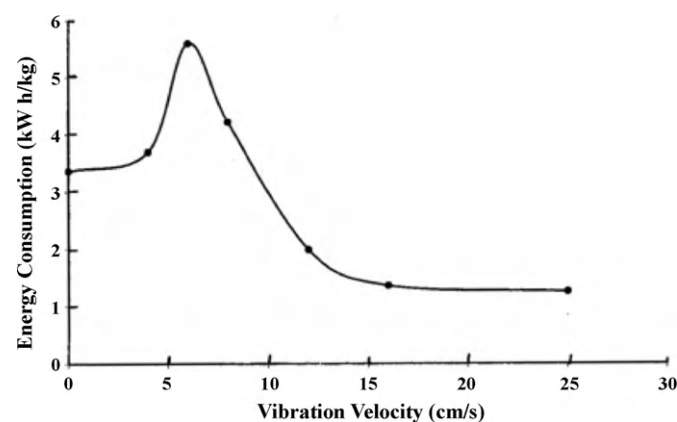
Fig. 14. Effect of vibration velocity on the energy consumption of FeSO 4 oxidation.
