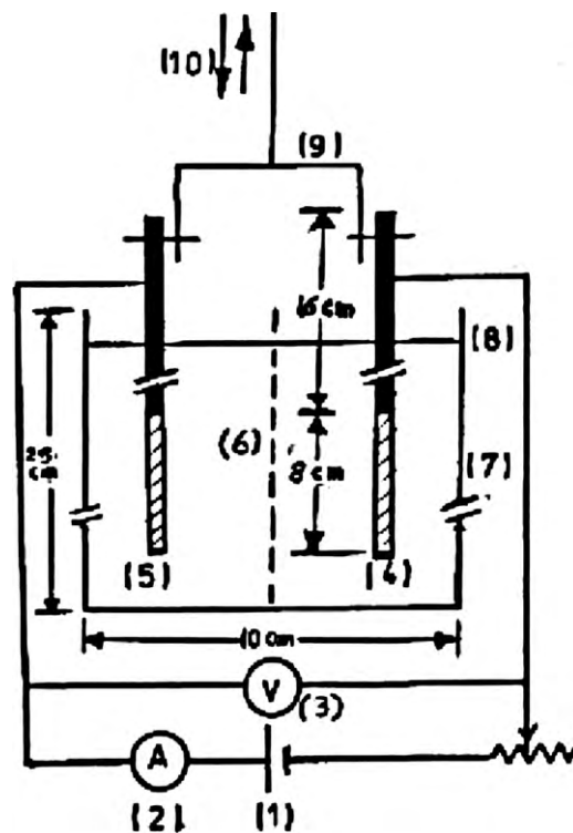
Fig. 1. Cell and electrical circuit used for constant current electrolysis. (1) Power supply; (2) multirange ammeter; (3) voltmeter; (4) cathode; (5) anode; (6) porous diaphragm; (7) Plexiglas cell; (8) electrolyte level; (9) plastic holder; (10) To vibrator.
